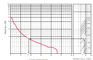
PERFORMANCE DIAGRAM
