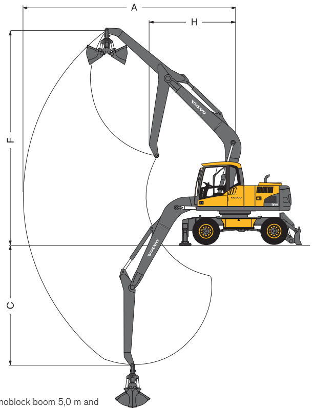
Monoblock boom 5,0 m and grab arm 2,95 m
